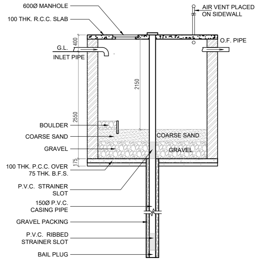
SECTION THROUGH E-E
