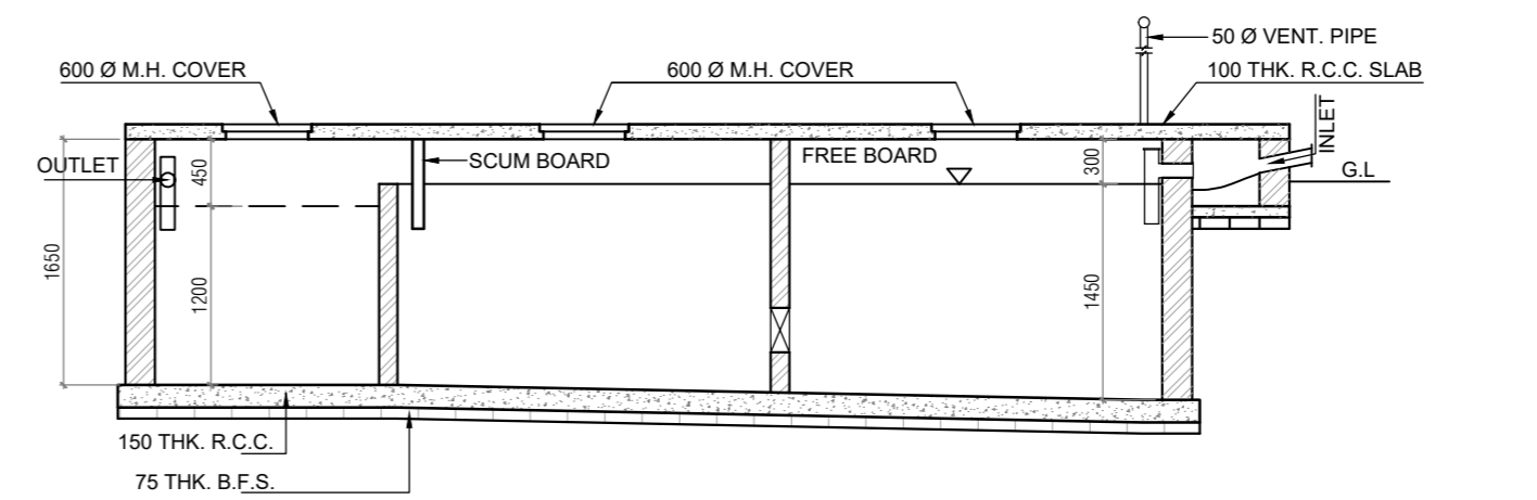
SECTION THROUGH D-D
