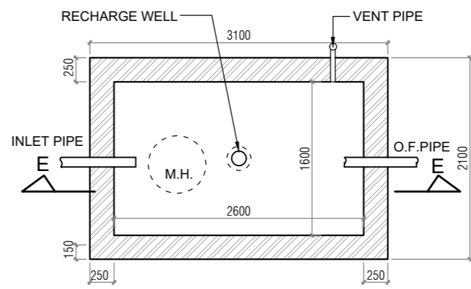
PLAN DETAIL OF RAIN WATER RECHARGE TANK SCALE 1:50
